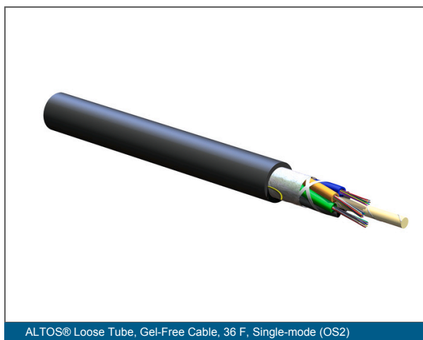
ALTOS® Loose Tube, Gel-Free Cable, 36 F, Single-mode (OS2)
