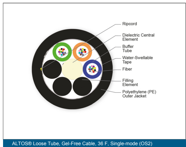
ALTOS® Loose Tube, Gel-Free Cable, 36 F, Single-mode (OS2)
